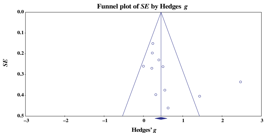
Figure 2 — Funnel plot of effect sizes from individual studies.
